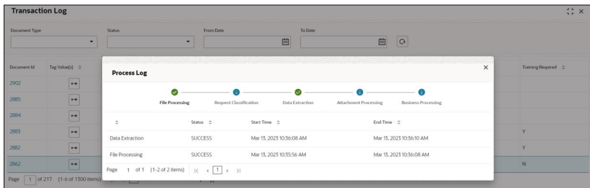
Figure 292: Execution Flow
